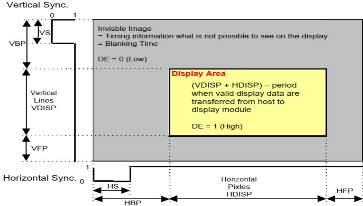
General timing diagram
