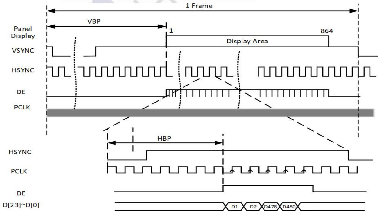
RGB (800RGB x 480) timing diagram
